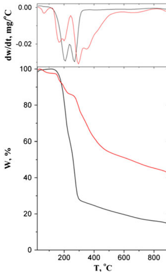
Figure 5. TG/DTG curves of SB (black line) and SB-Cu(II) complex (red line)
