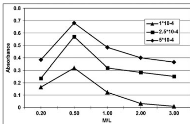
Figure 2. Adsorbance versus molar ratio M/L for SB/Cu(II) complex
