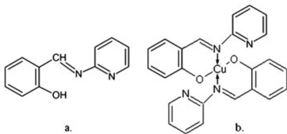
Figure 1. Structure of the ligand (a) and complex (b)
