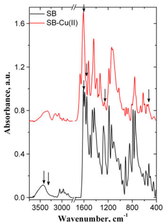
Figure 3. FT-IR spectra of SB and SB-Cu(II) complex
