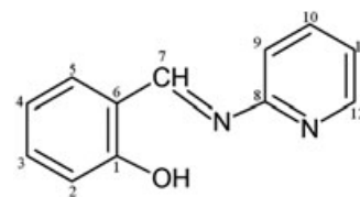
Figure 4. Numbering of carbon atoms in SB
