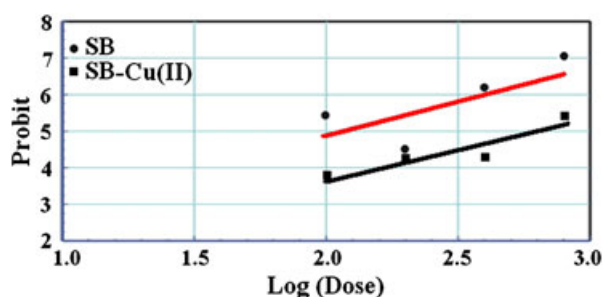
Figure 6. Regression line for SB and SB-Cu(II)
