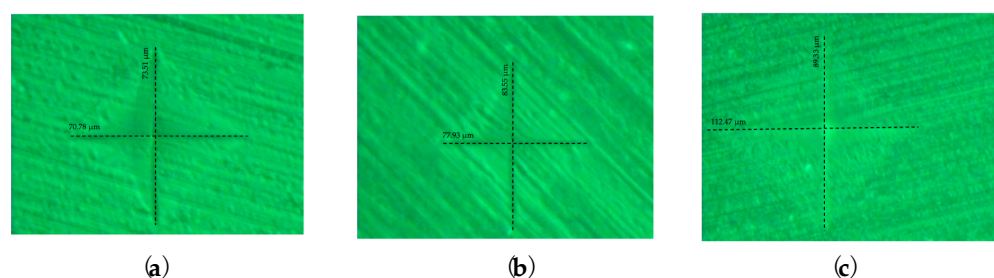
Figure 7. The impressions of the penetrator on the surface of the samples: (a) Group 1.2—Sample 3 heat-cured; (b) Group 2.2—Sample 2 CAD/CAM milled; (c) Group 3.2—Sample 8 3D printed.
