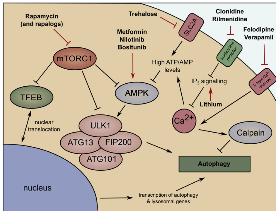
Fig. 2. Small molecule inducers of autophagy and their mechanisms of action. Autophagy is regulated by the mTORC1 pathway, and inhibitors of mTORC1, including rapamycin and rapalogs, are among the best-studied class of autophagy inducers. Other modulators are classed as mTOR-independent and act on various targets, including AMPK, IP 3 signaling, and Ca 2+ signaling.
