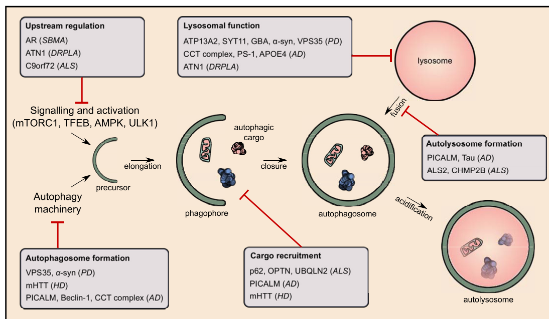
Fig. 1. Defective autophagy and neurodegenerative disease. A number of risk genes linked to neurodegenerative diseases play a role in the autophagy pathway. These genes intersect with the autophagy pathway at many different stages, as indicated here. Disruptions to autophagy caused by pathogenic changes to the relevant genes may contribute to disease pathogenesis.
