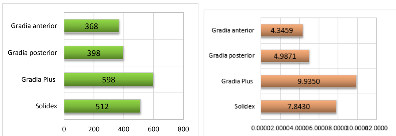
Figure 3, 4. Aspect of hardness and elasticity moduls at biomaterials analysed
